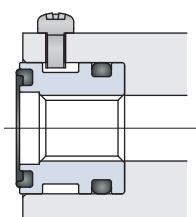
Machine side
