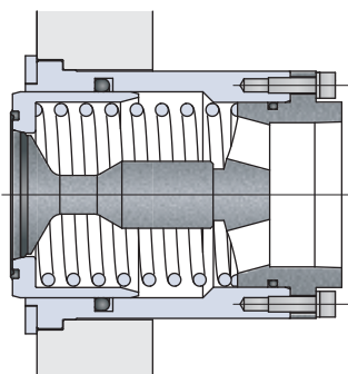
Machine side
