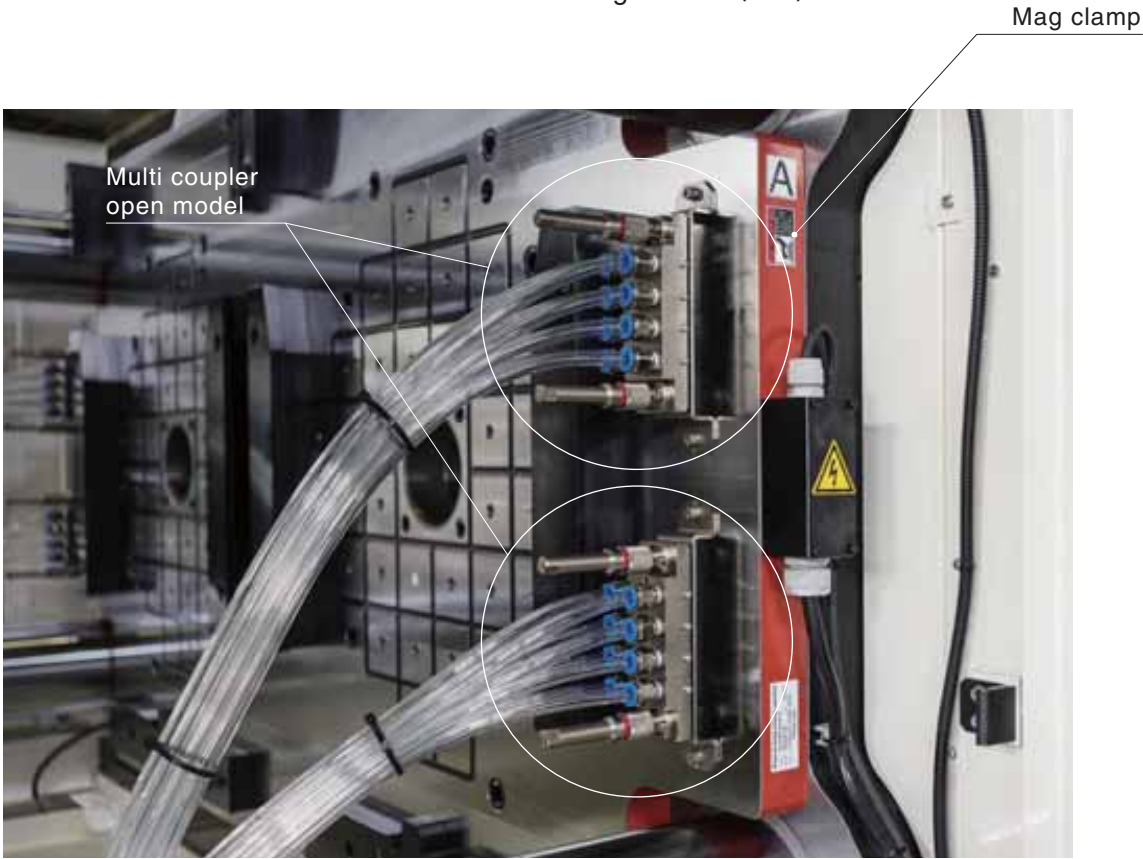
For temperature control & air valve gate
