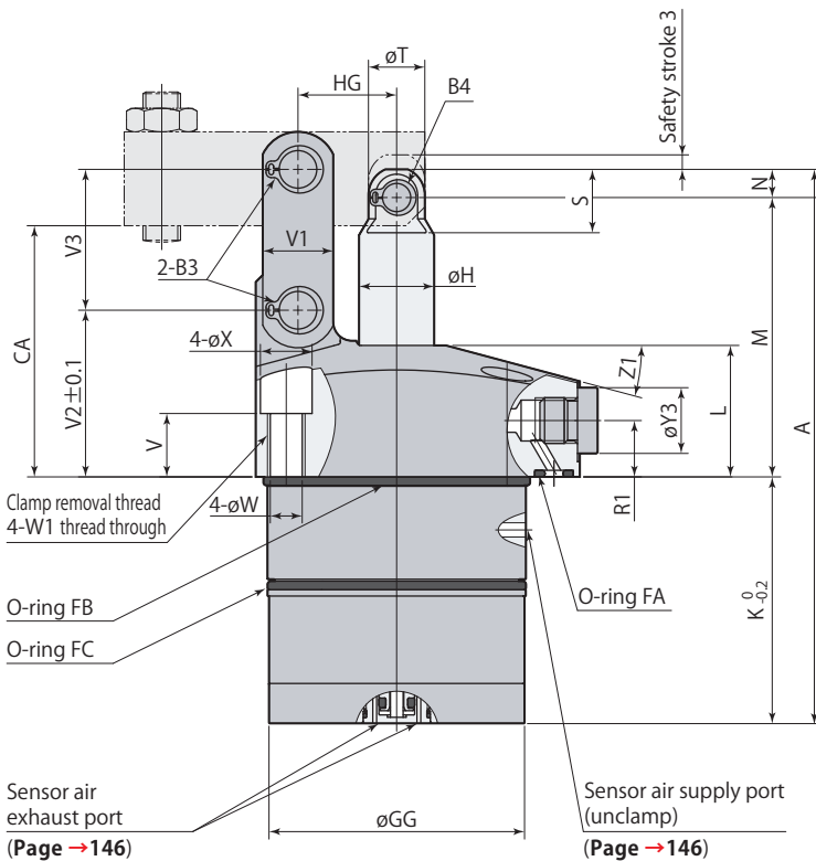
Clamp
