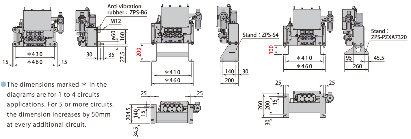
Anti vibration rubber (option) model ZPS-B6
